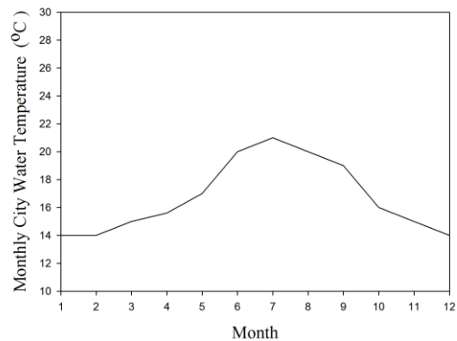
Fig. 7 Monthly city water temperature profile in Mosul city.
