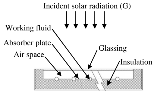
Fig. 1 Schematic diagram of flat-plate solar collector
