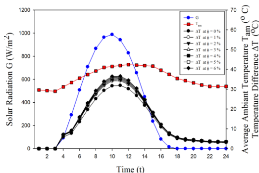
Fig. 5 Variation of hourly solar radiation on the solar collectors, ambient temperature and working fluid temperature differences as a function of nanoparticle volume fraction during a typical day in July.
