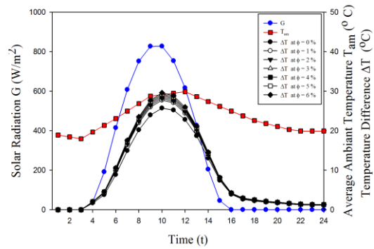
Fig. 6 Variation of hourly solar radiation on the solar collectors, ambient temperature and working fluid temperature differences as a function of nanoparticle volume fraction during a typical day in October.
