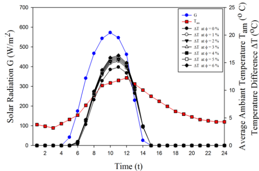
Fig. 3 Variation of hourly solar radiation on the solar collectors, ambient temperature and working fluid temperature differences as a function of nanoparticle volume fraction during a typical day in January.
