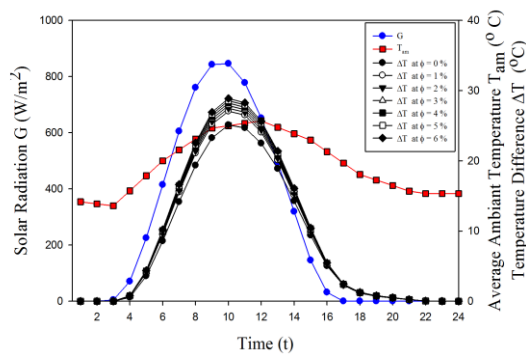
Fig. 4 Variation of hourly solar radiation on the solar collectors, ambient temperature and working fluid temperature differences as a function of nanoparticle volume fraction during a typical day in April.
