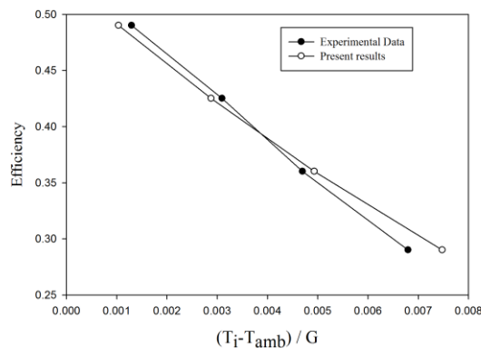
Fig. 2 NBFPS model validation.
